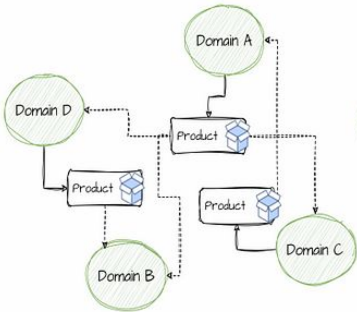
Data Mesh
